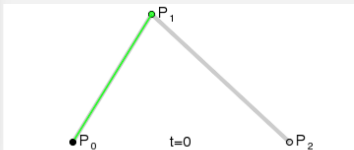
Bézier Curve
